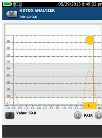
High Definition Time Domain Cross talk (HTDXT) shows the far end connection is clearly the issue
